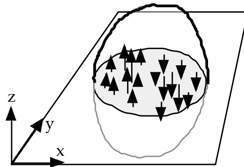
Figure 1. A schematic eddy. Main features are that an outline can be defined and its internal structure is simple. This is illustrated here by showing the vertical velocity not random but organized into well-defined areas of updraft and downdraft.
